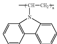
PVCz
