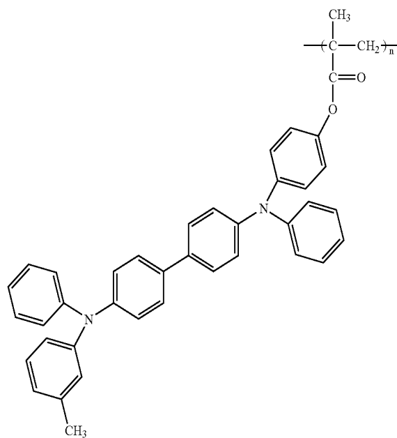
TPD-PMMA
