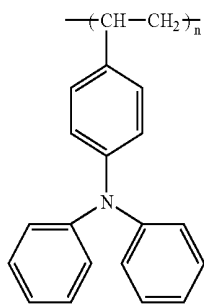
DPA-PS
