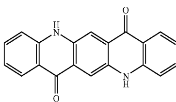
Quinacridone
