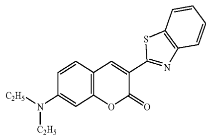
Coumarin6
